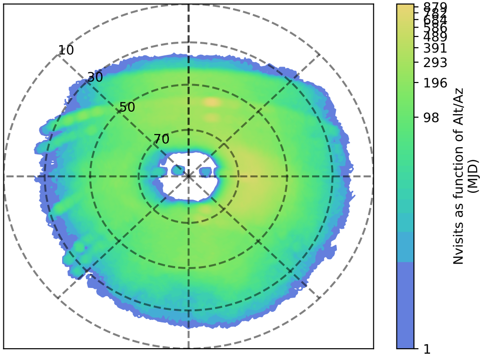
ddf_acor_sf25_lsf30_lsr20_v3.4_10yrs u: Nvisits as function of Alt/Az
