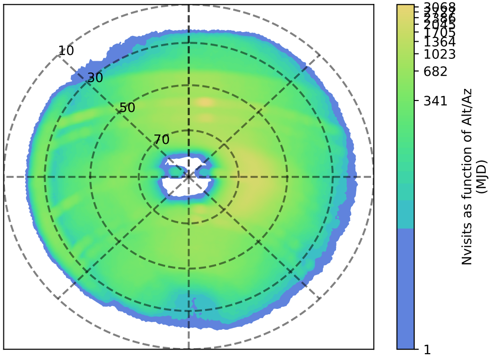
ddf_acor_sf25_ls30_lsr20_v3.4_10yrs r: Nvisits as function of Alt/Az
