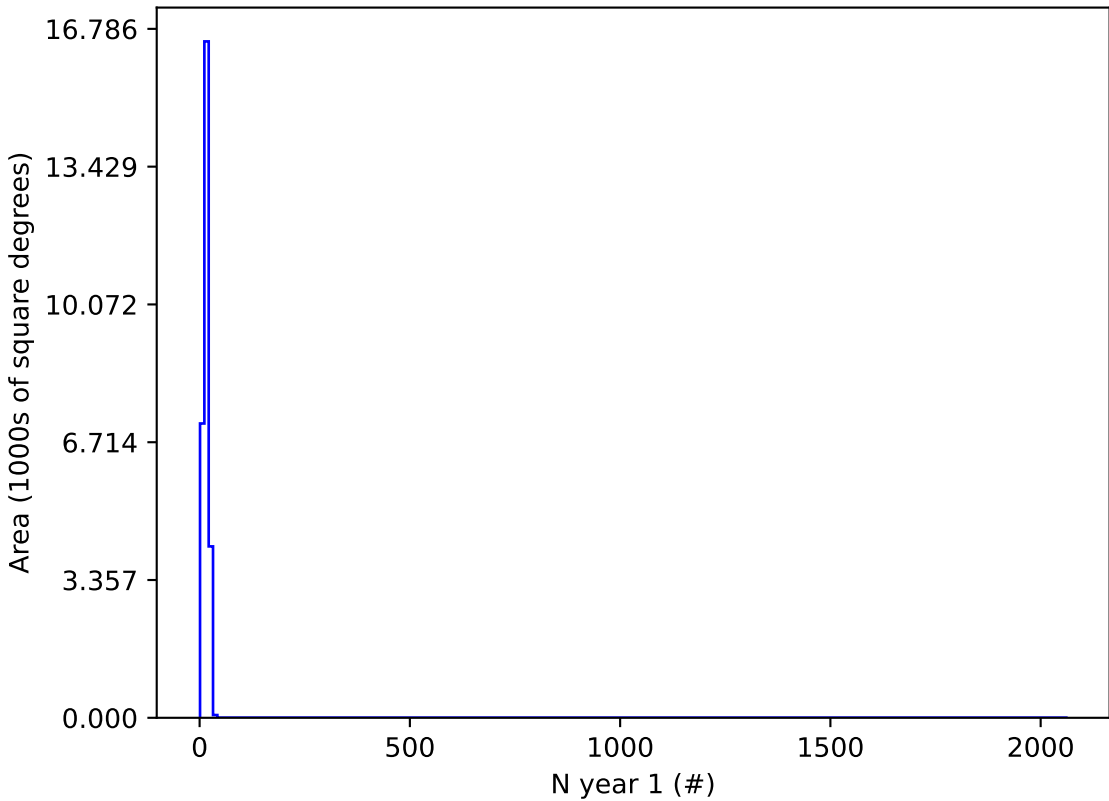
ddf_acor_sf25_lsf30_lsr20_v3.4_10yrs r and night < 365: N year 1
