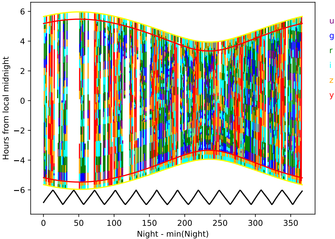
ddf_acor_sf25_lsf30_lsr20_v3.4_10yrs year 8-9: Hourglass
