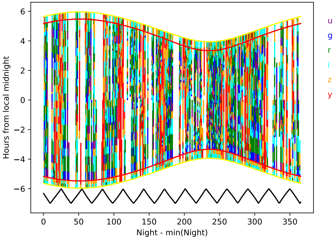
ddf_acor_sf25_lsf30_lsr20_v3.4_10yrs year 7-8: Hourglass
