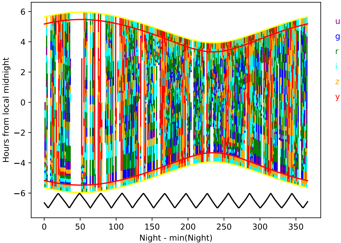
ddf_acor_sf25_lsf30_lsr20_v3.4_10yrs year 2-3: Hourglass
