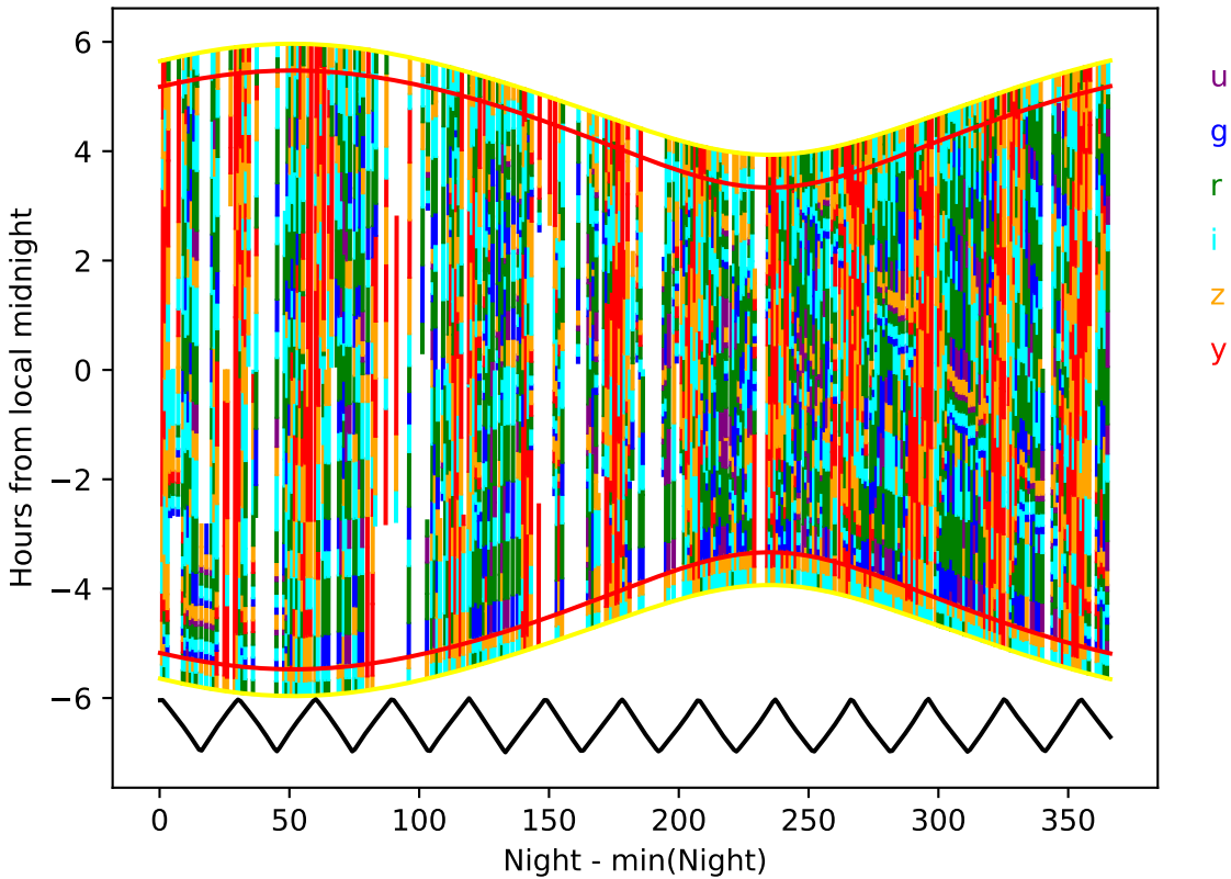
ddf_acor_sf25_lsf30_lsr20_v3.4_10yrs year 1-2: Hourglass
