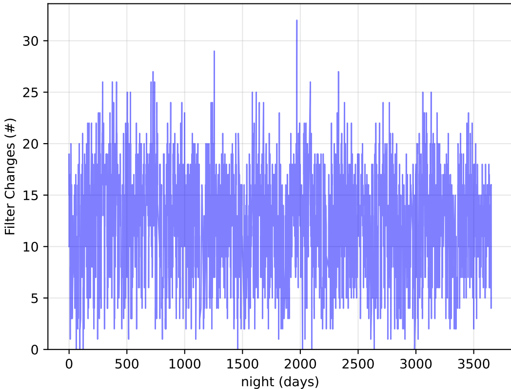
ddf_acor_sf25_ls30_lsr20_v3.4_10yrs : Filter Changes
