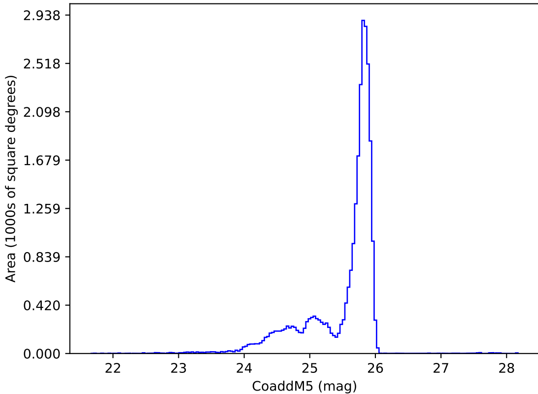
ddf_acor_sf25_lsf30_lsr20_v3.4_10yrs z: CoaddM5
