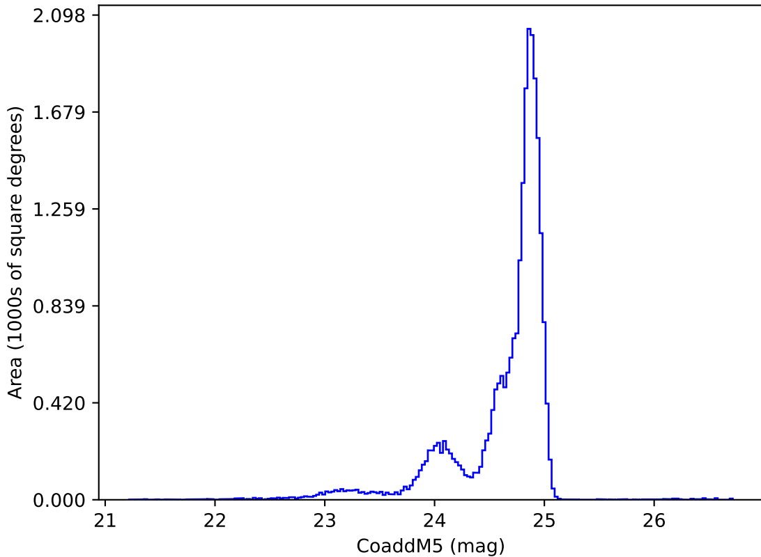
ddf_acor_sf25_lsf30_lsr20_v3.4_10yrs y: CoaddM5
