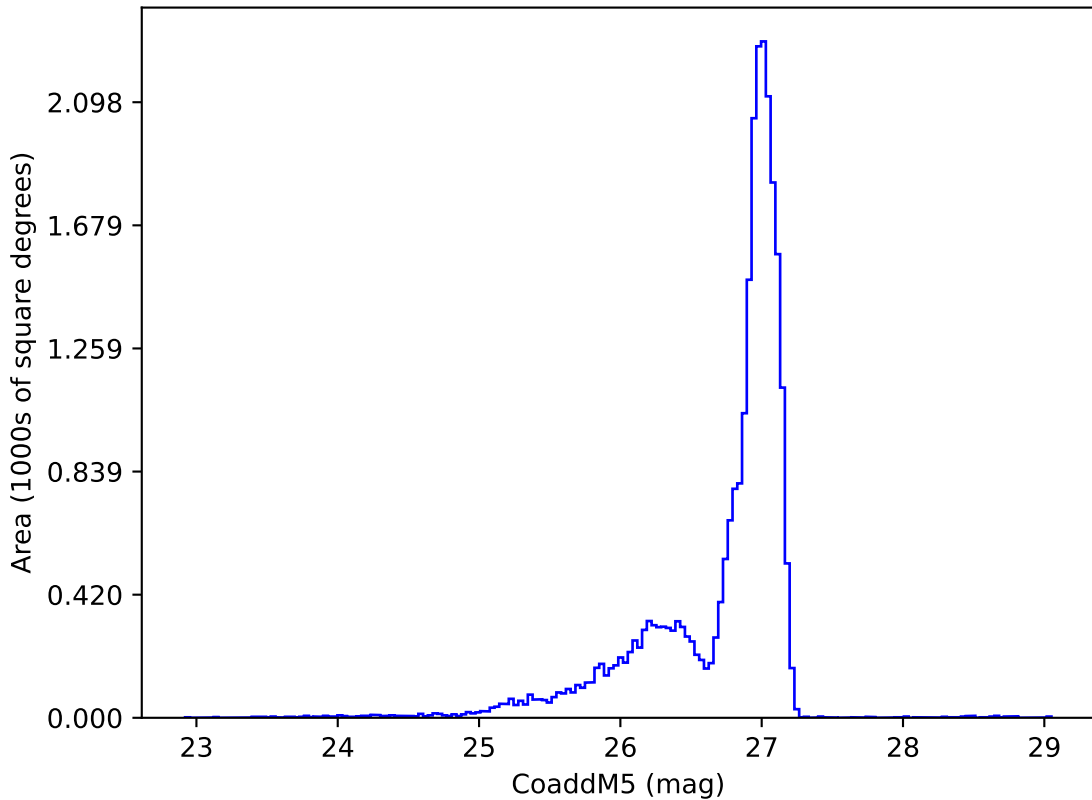
ddf_acor_sf25_lsf30_lsr20_v3.4_10yrs r: CoaddM5
