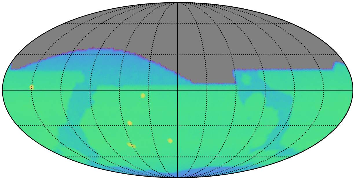
ddf_acor_sf25_lsf30_lsr20_v3.4_10yrs i: CoaddM5
