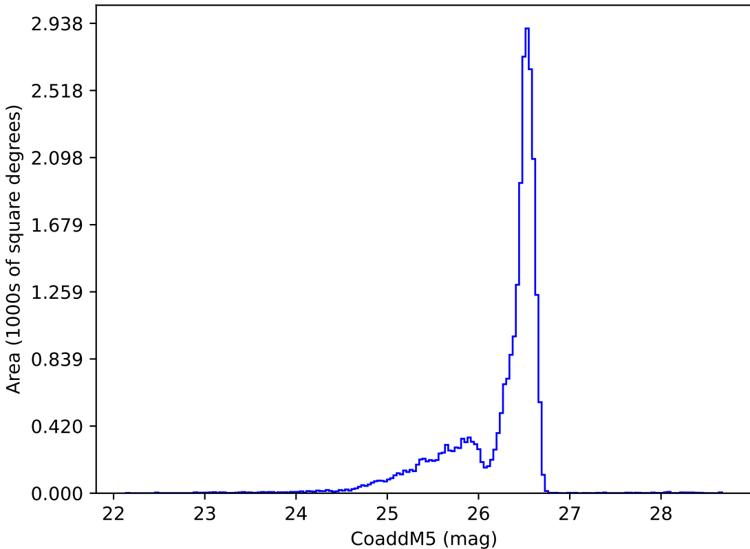
ddf_acor_sf25_lsf30_lsr20_v3.4_10yrs i: CoaddM5
