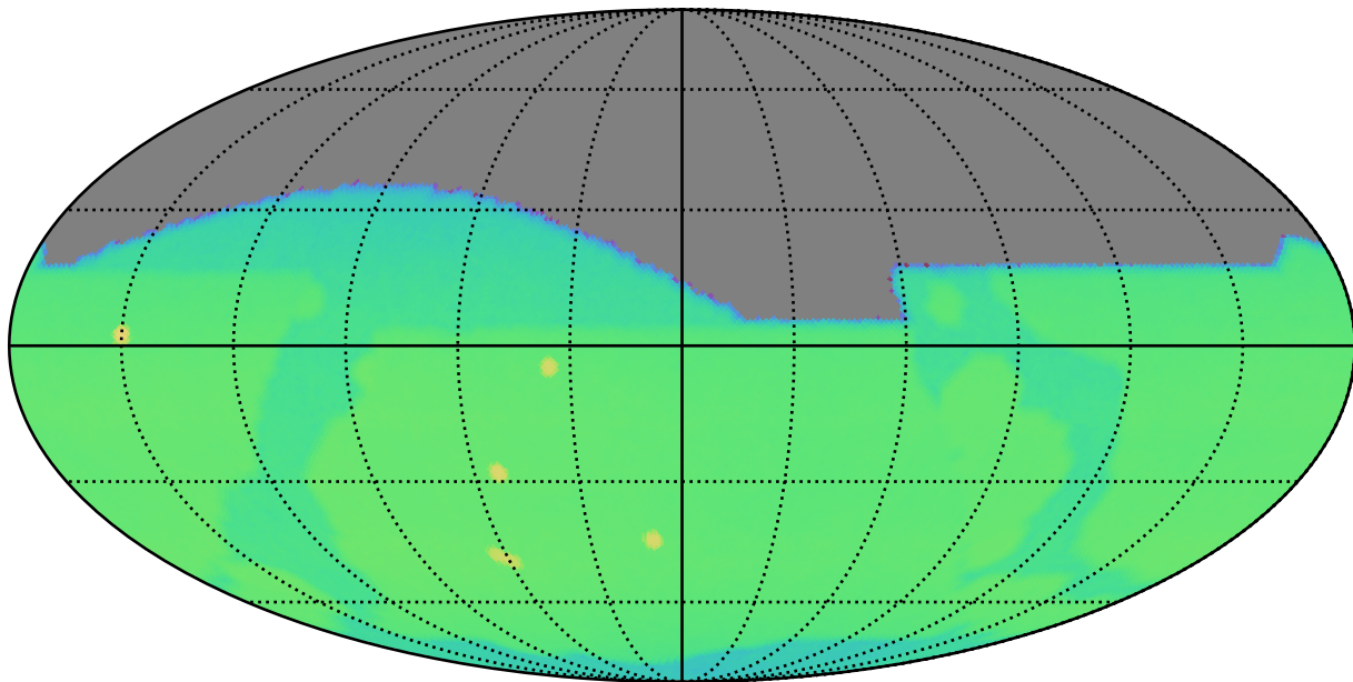
ddf_acor_sf25_lsf30_lsr20_v3.4_10yrs : CoaddM5
