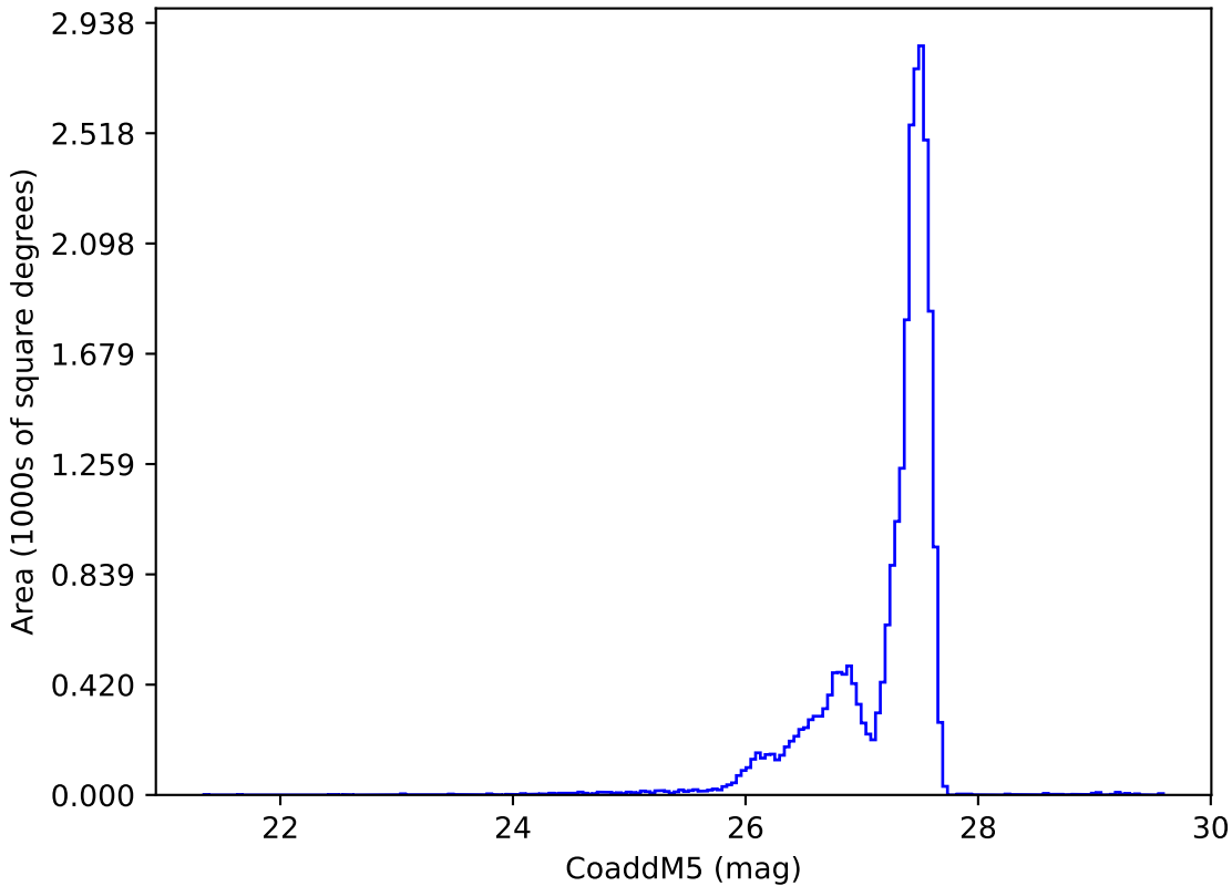
ddf_acor_sf25_lsf30_lsr20_v3.4_10yrs : CoaddM5
