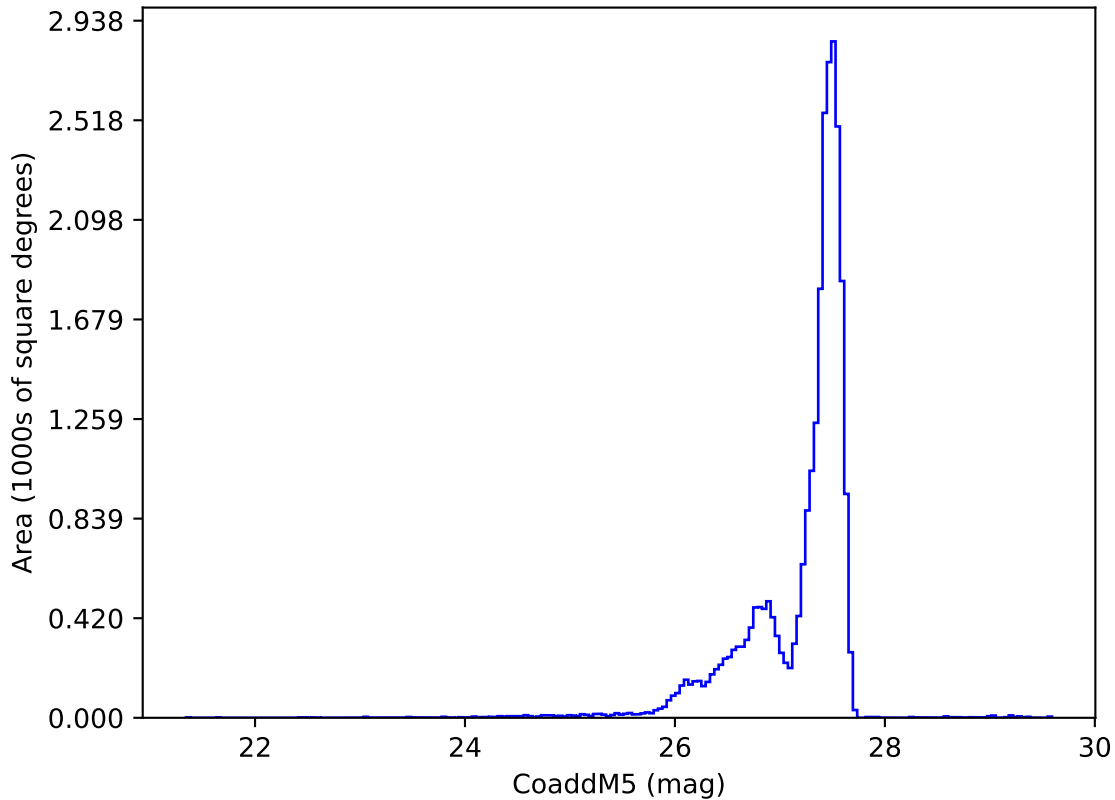
ddf_acor_sf25_lsf30_lsr20_v3.4_10yrs : CoaddM5
