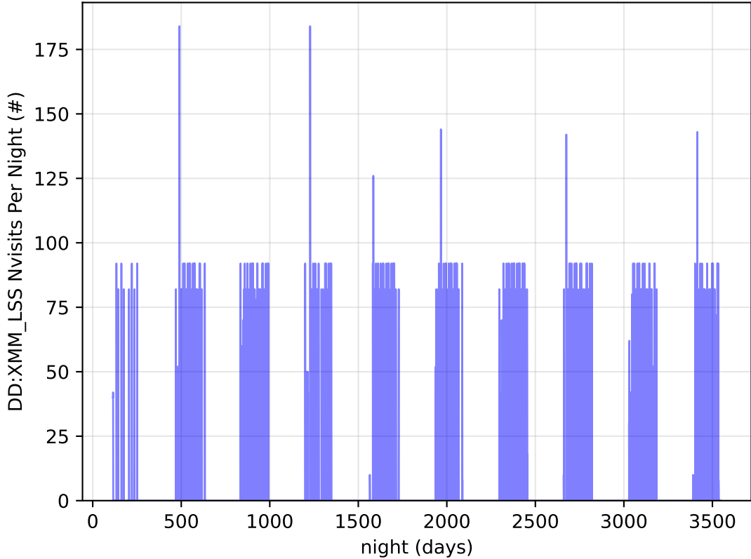
ddf_acor_sf25_lsf30_lsr20_v3.4_10yrs all bands: DD:XMM_LSS Nvisits Per Night
