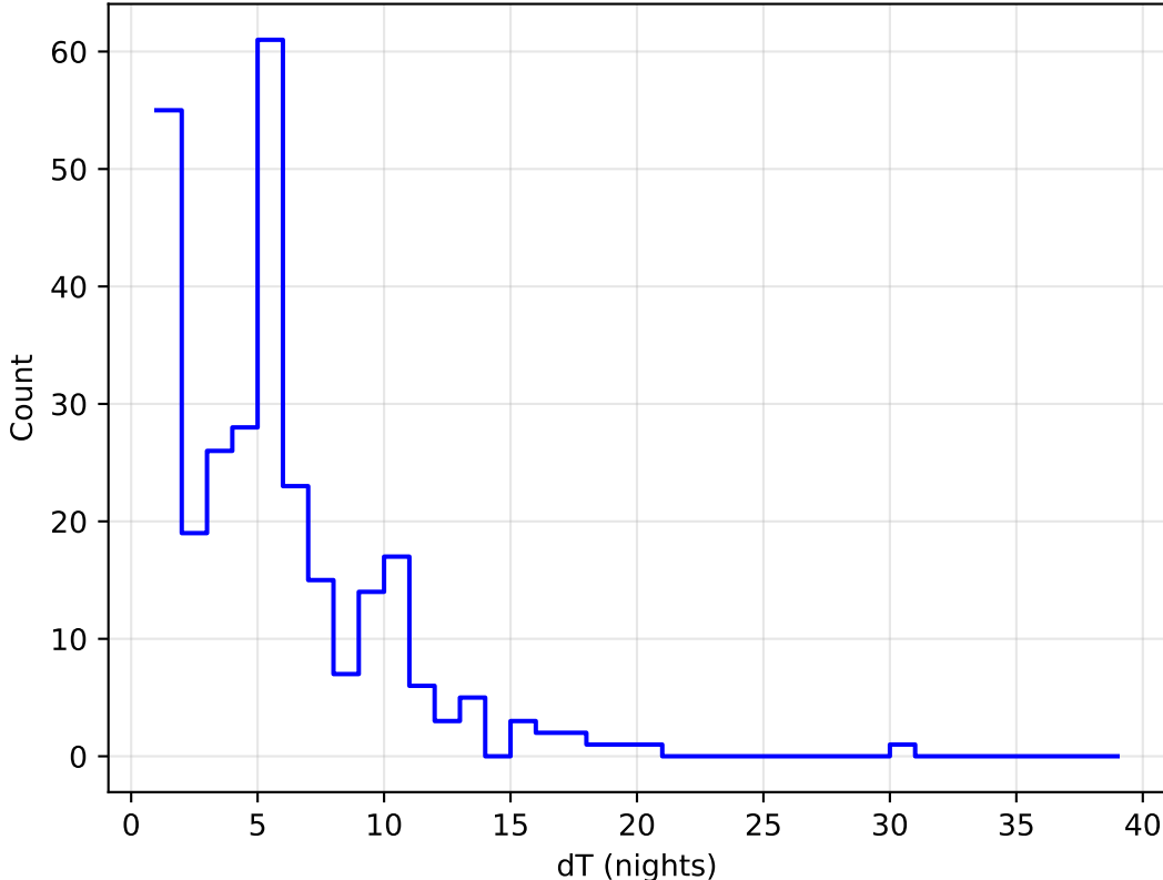
ddf_acor_sf25_lsf30_lsr20_v3.4_10yrs all bands: DD:XMM_LSS Delta Nights Histogram
