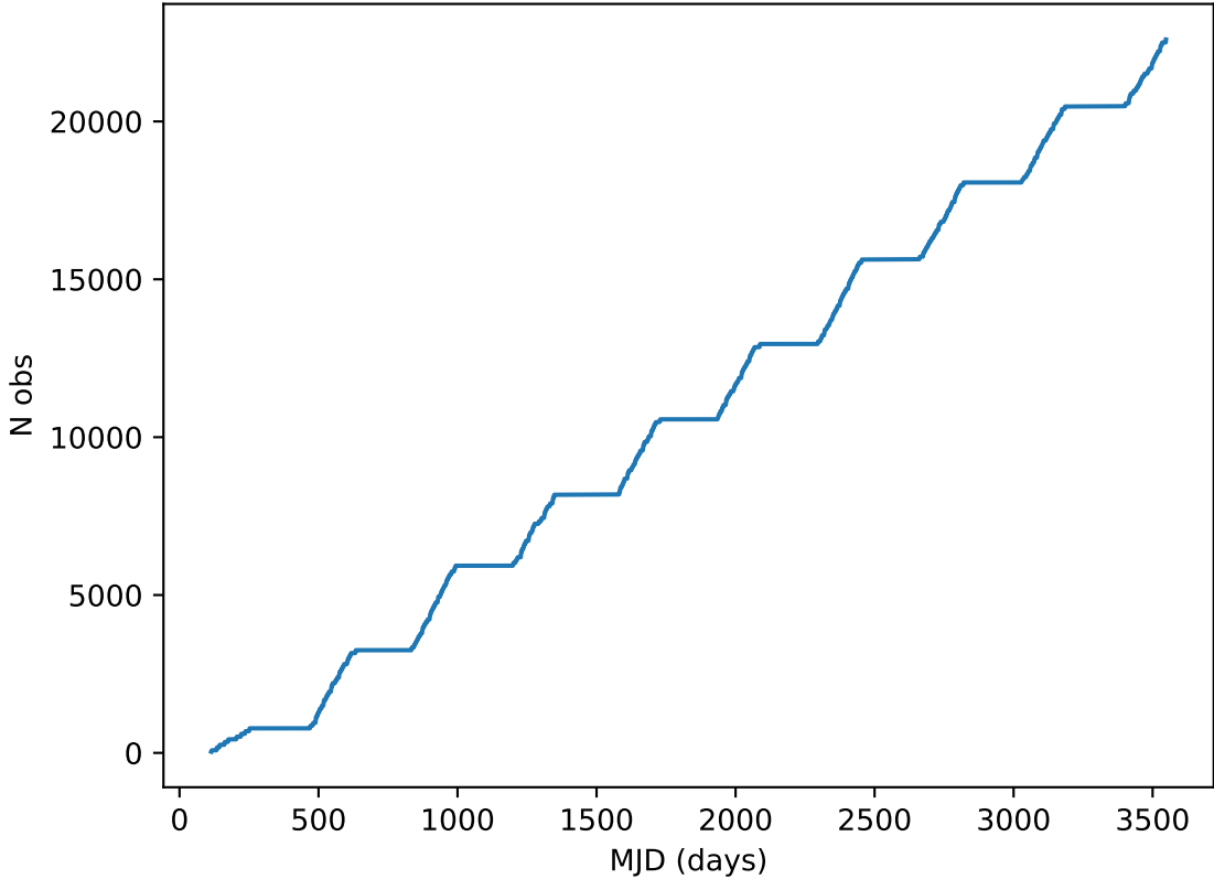
ddf_acor_sf25_lsf30_lsr20_v3.4_10yrs all bands: DD:XMM_LSS Cumulative NVisits
