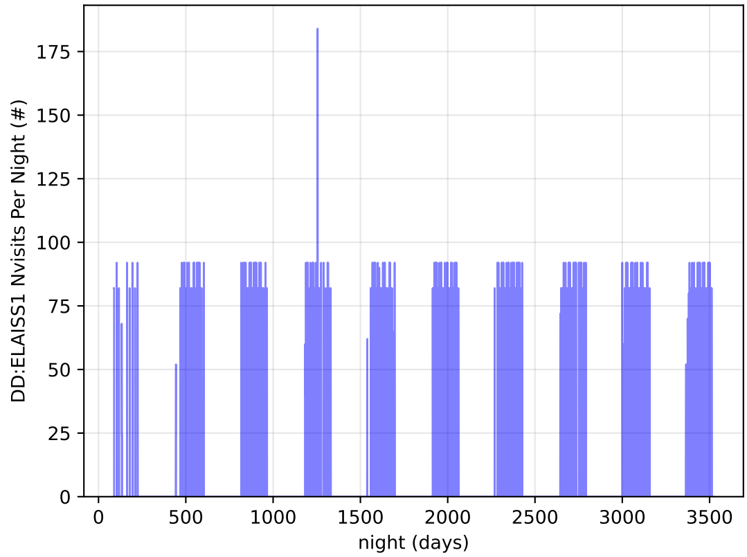
ddf_acor_sf25_lsf30_lsr20_v3.4_10yrs all bands: DD:ELAISS1 Nvisits Per Night
