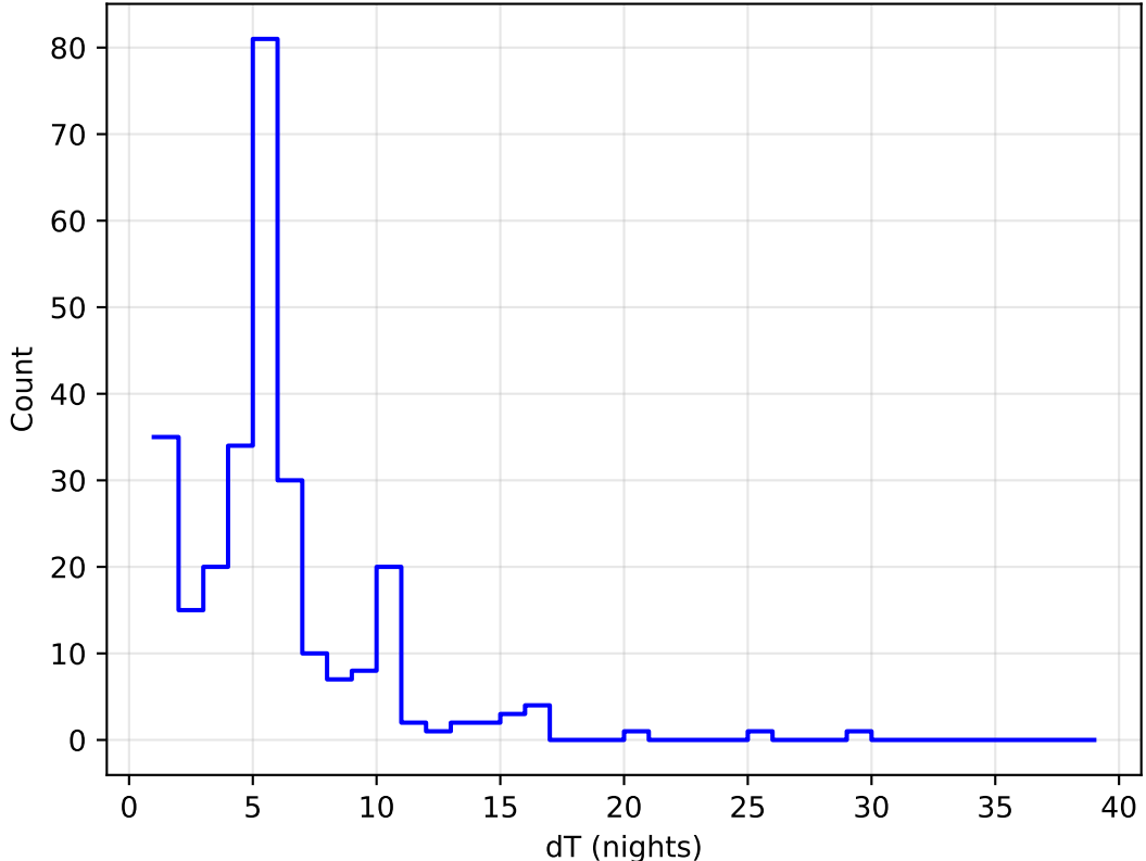
ddf_acor_sf25_lsf30_lsr20_v3.4_10yrs all bands: DD:ELAISS1 Delta Nights Histogram
