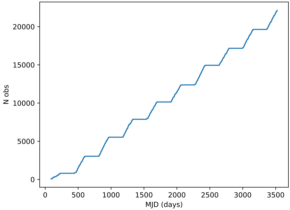
ddf_acor_sf25_lsf30_lsr20_v3.4_10yrs all bands: DD:ELAISS1 Cumulative NVisits
