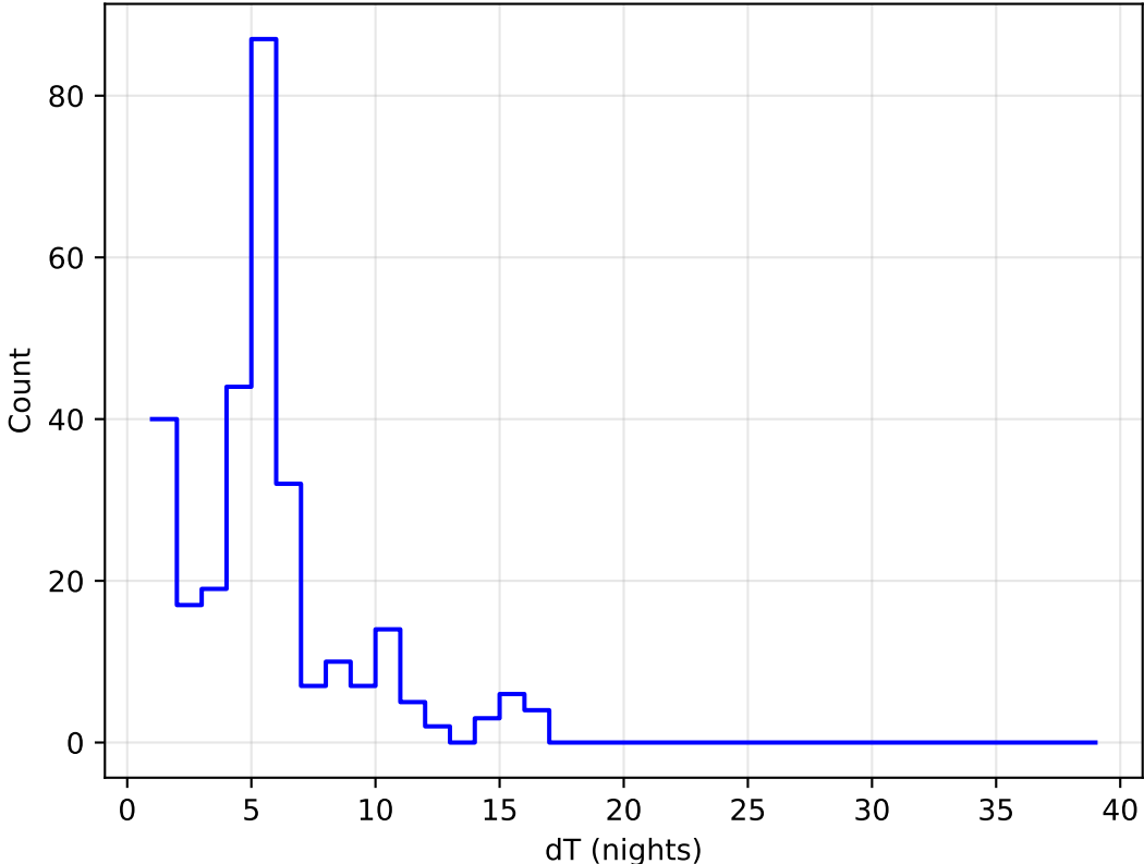
ddf_acor_sf25_lsf30_lsr20_v3.4_10yrs all bands: DD:EDFS Delta Nights Histogram
