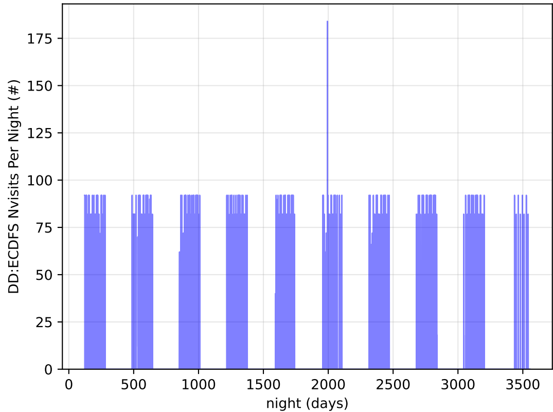
ddf_acor_sf25_lsf30_lsr20_v3.4_10yrs all bands: DD:ECDFS Nvisits Per Night
