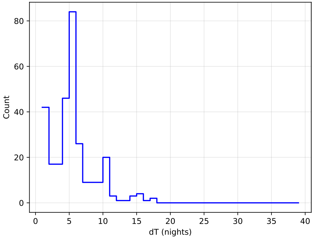
ddf_acor_sf25_lsf30_lsr20_v3.4_10yrs all bands: DD:ECDFS Delta Nights Histogram
