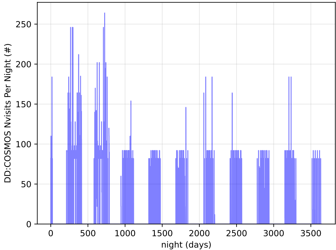
ddf_acor_sf25_lsf30_lsr20_v3.4_10yrs all bands: DD:COSMOS Nvisits Per Night
