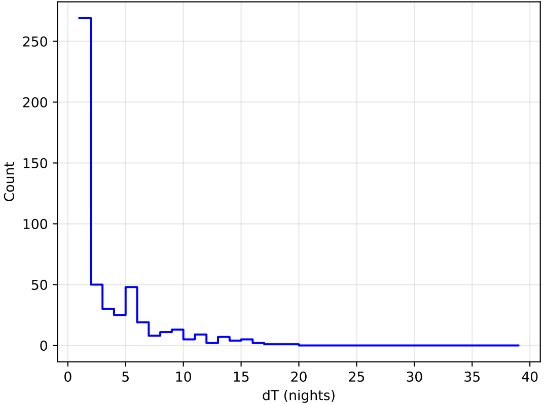
ddf_acor_sf25_Isf30_Isr20_v3.4_10yrs all bands: DD: COSMOS Delta Nights Histogram
