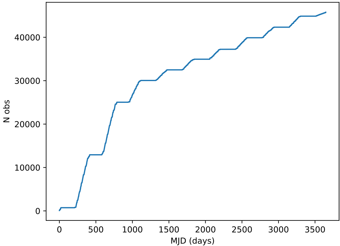
ddf_acor_sf25_lsf30_lsr20_v3.4_10yrs all bands: DD: COSMOS Cumulative NVisits
