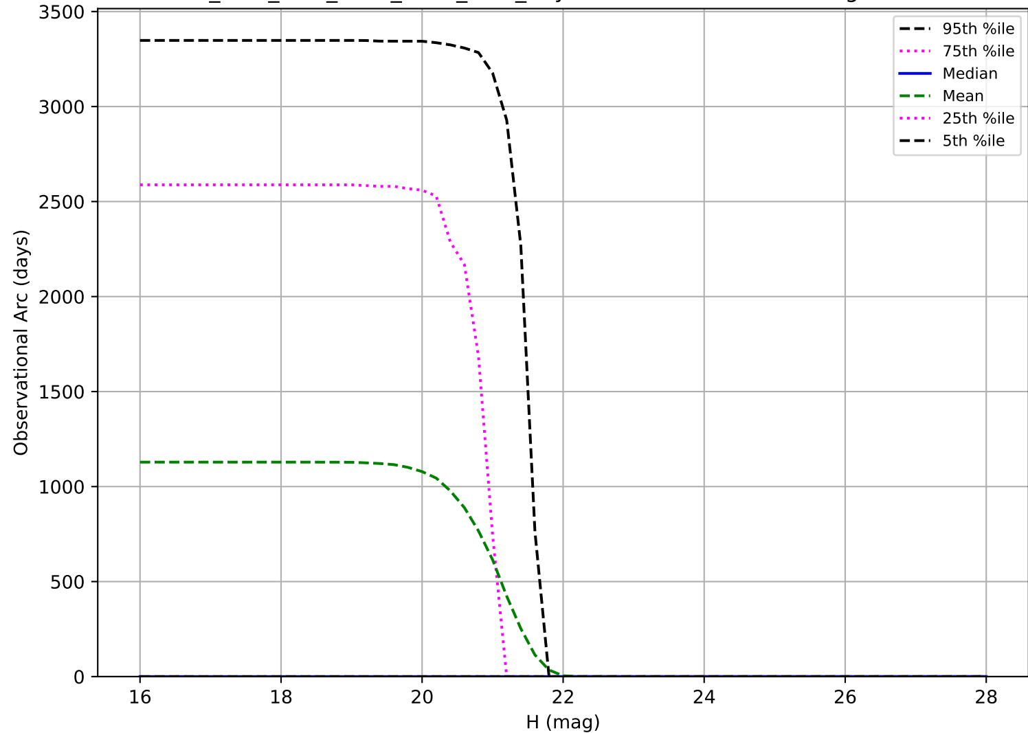
ddf_acor_sf25_lsf30_lsr10_v3.4_10yrs: Observational Arc Length Vatira
