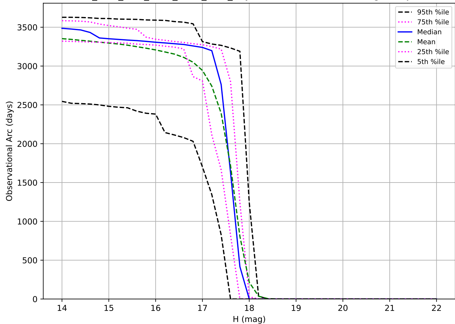
ddf_acor_sf25_lsf30_lsr10_v3.4_10yrs: Observational Arc Length Trojan
