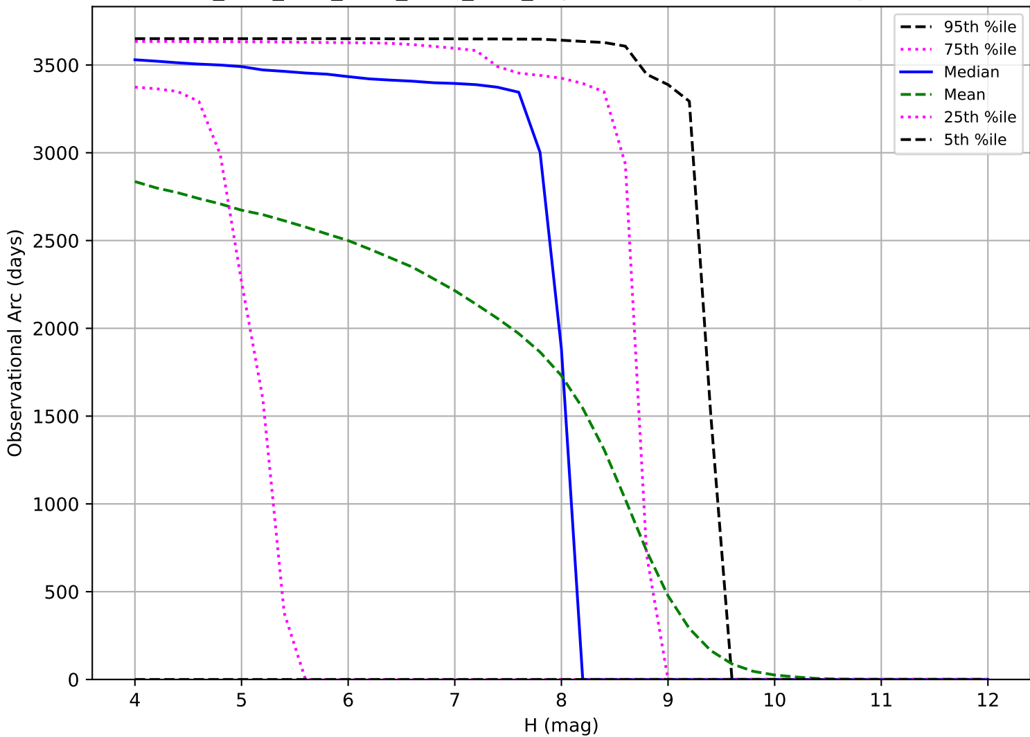
ddf_acor_sf25_lsf30_lsr10_v3.4_10yrs: Observational Arc Length TNO
