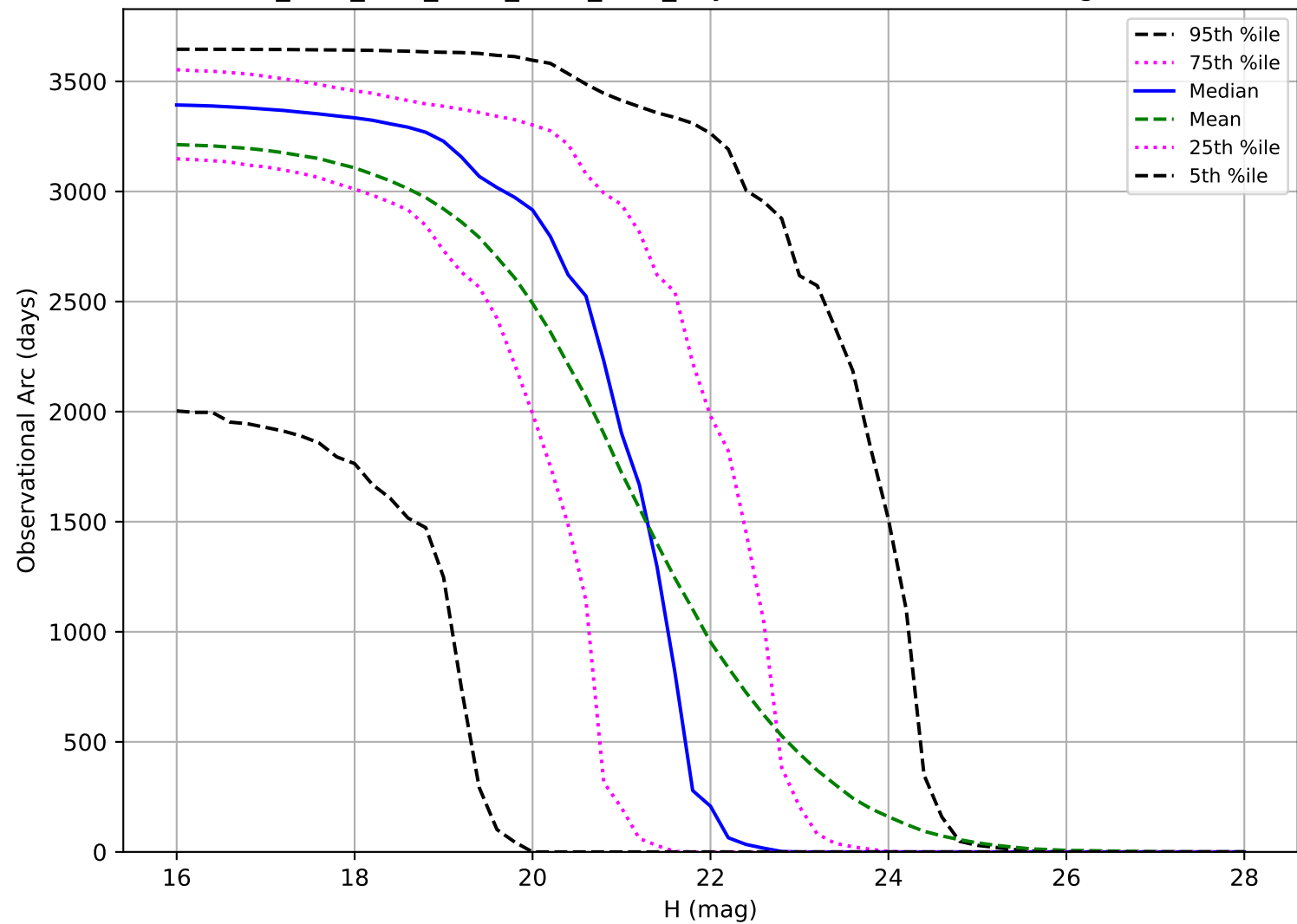
ddf_acor_sf25_lsf30_lsr10_v3.4_10yrs: Observational Arc Length PHA
