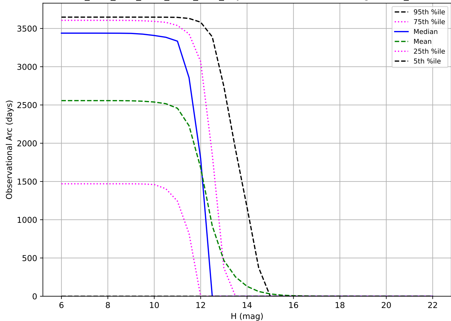
ddf_acor_sf25_lsf30_lsr10_v3.4_10yrs: Observational Arc Length OCC_r20
