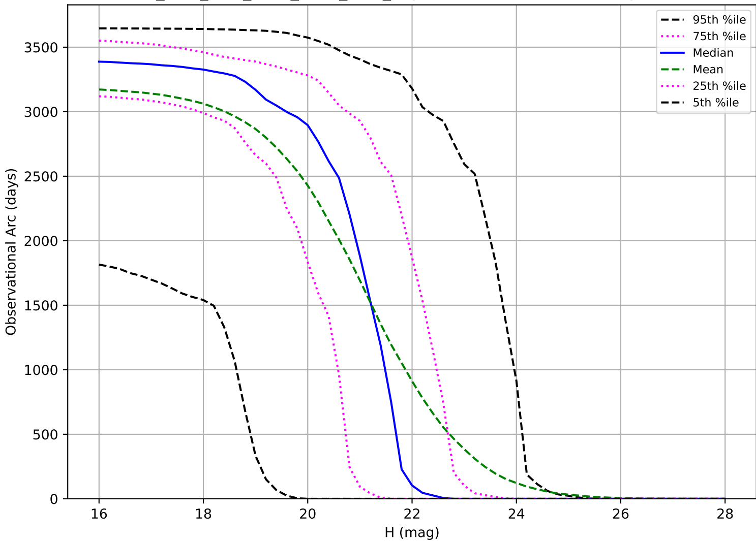
ddf_acor_sf25_lsf30_lsr10_v3.4_10yrs: Observational Arc Length NEO
