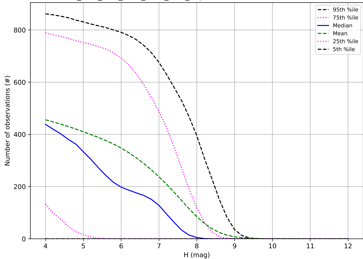
ddf_acor_sf25_lsf30_lsr10_v3.4_10yrs: Number of observations TNO
