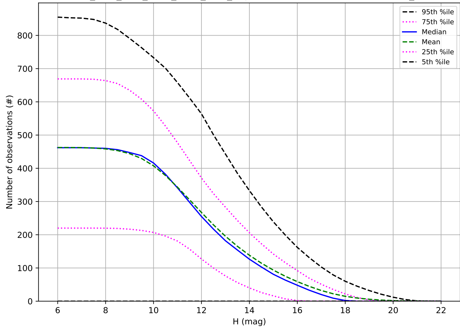
ddf_acor_sf25_lsf30_lsr10_v3.4_10yrs: Number of observations OCC_r5
