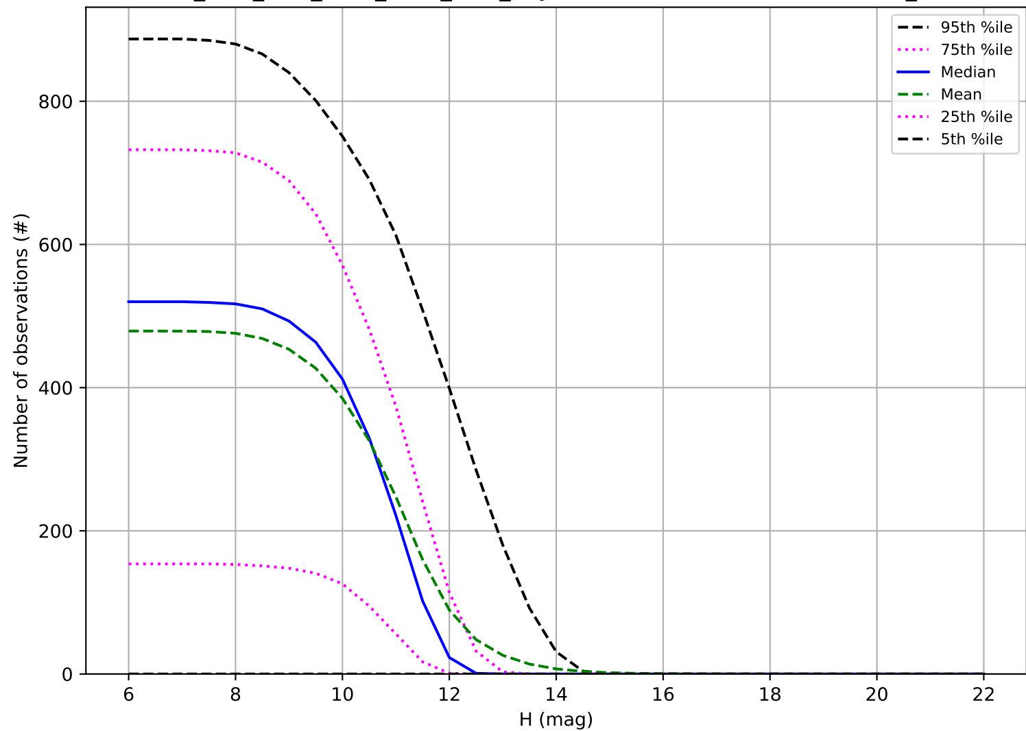
ddf_acor_sf25_lsf30_lsr10_v3.4_10yrs: Number of observations OCC_r20
