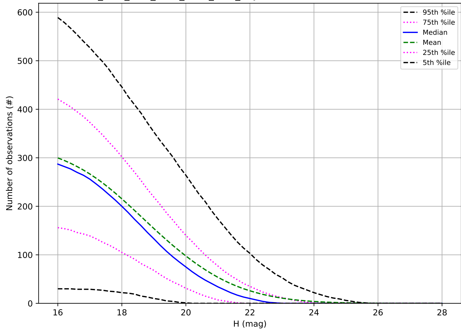
ddf_acor_sf25_lsf30_lsr10_v3.4_10yrs: Number of observations NEO
