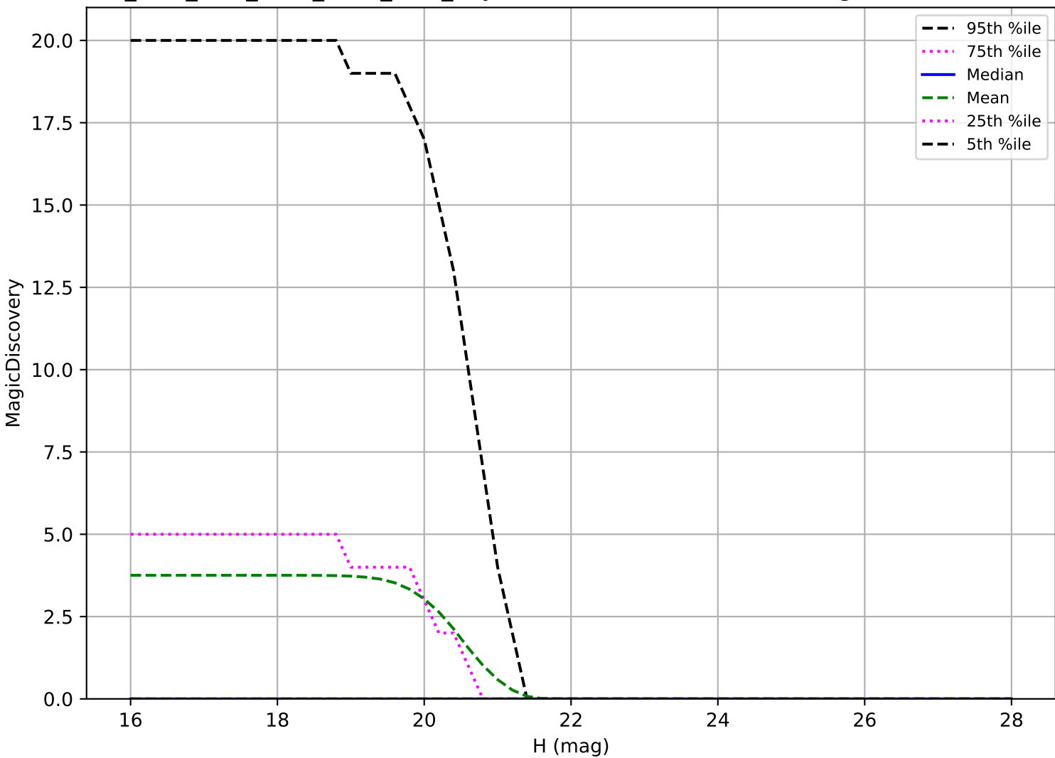
ddf_acor_sf25_lsf30_lsr10_v3.4_10yrs: Vatra 6 detections in 60 nights detection loss
