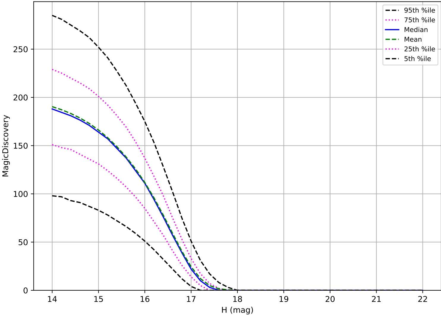
ddf_acor_sf25_lsf30_lsr10_v3.4_10yrs: Trojan 6 detections in 60 nights detection loss
