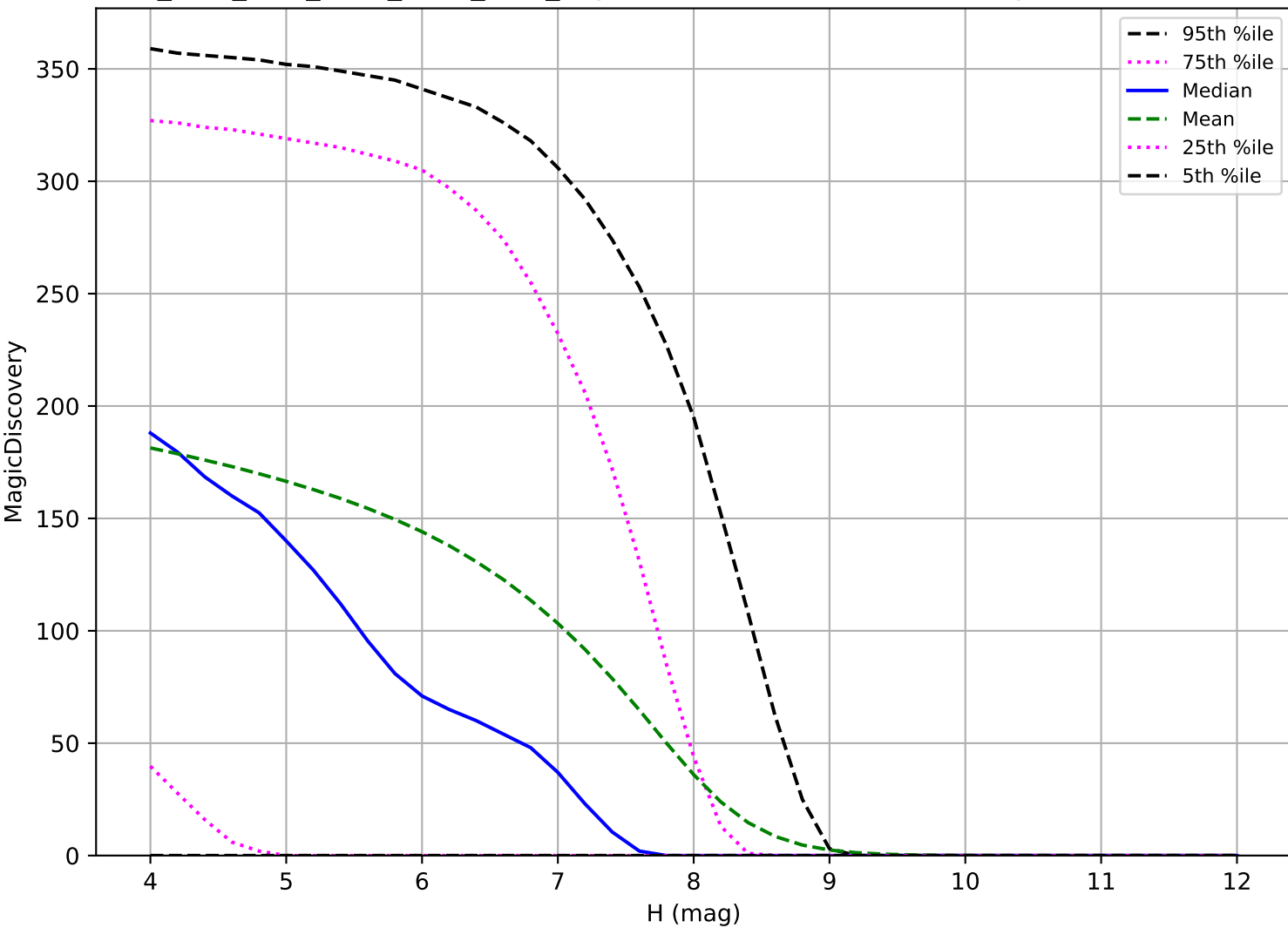
ddf_acor_sf25_lsf30_lsr10_v3.4_10yrs: TNO 6 detections in 60 nights detection loss
