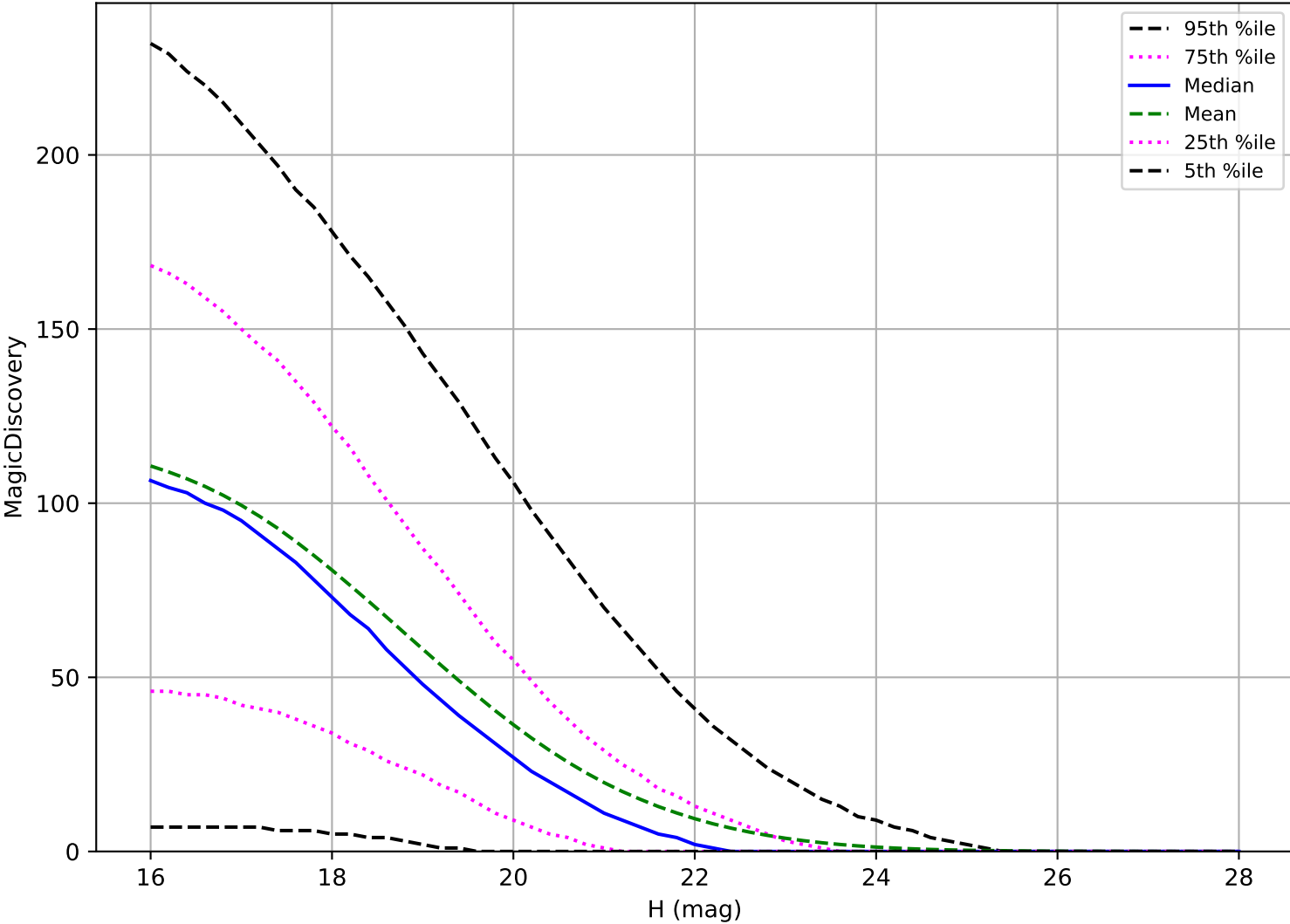
ddf_acor_sf25_lsf30_lsr10_v3.4_10yrs: PHA 6 detections in 60 nights detection loss
