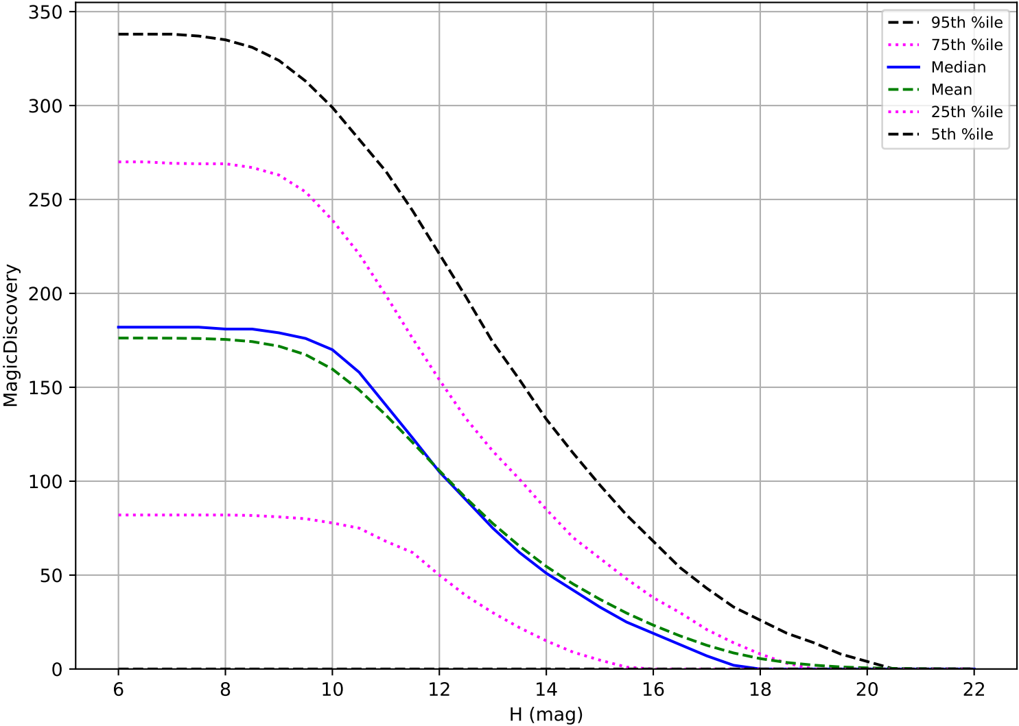
ddf_acor_sf25_lsf30_lsr10_v3.4_10yrs: OCC_r5 6 detections in 60 nights detection loss
