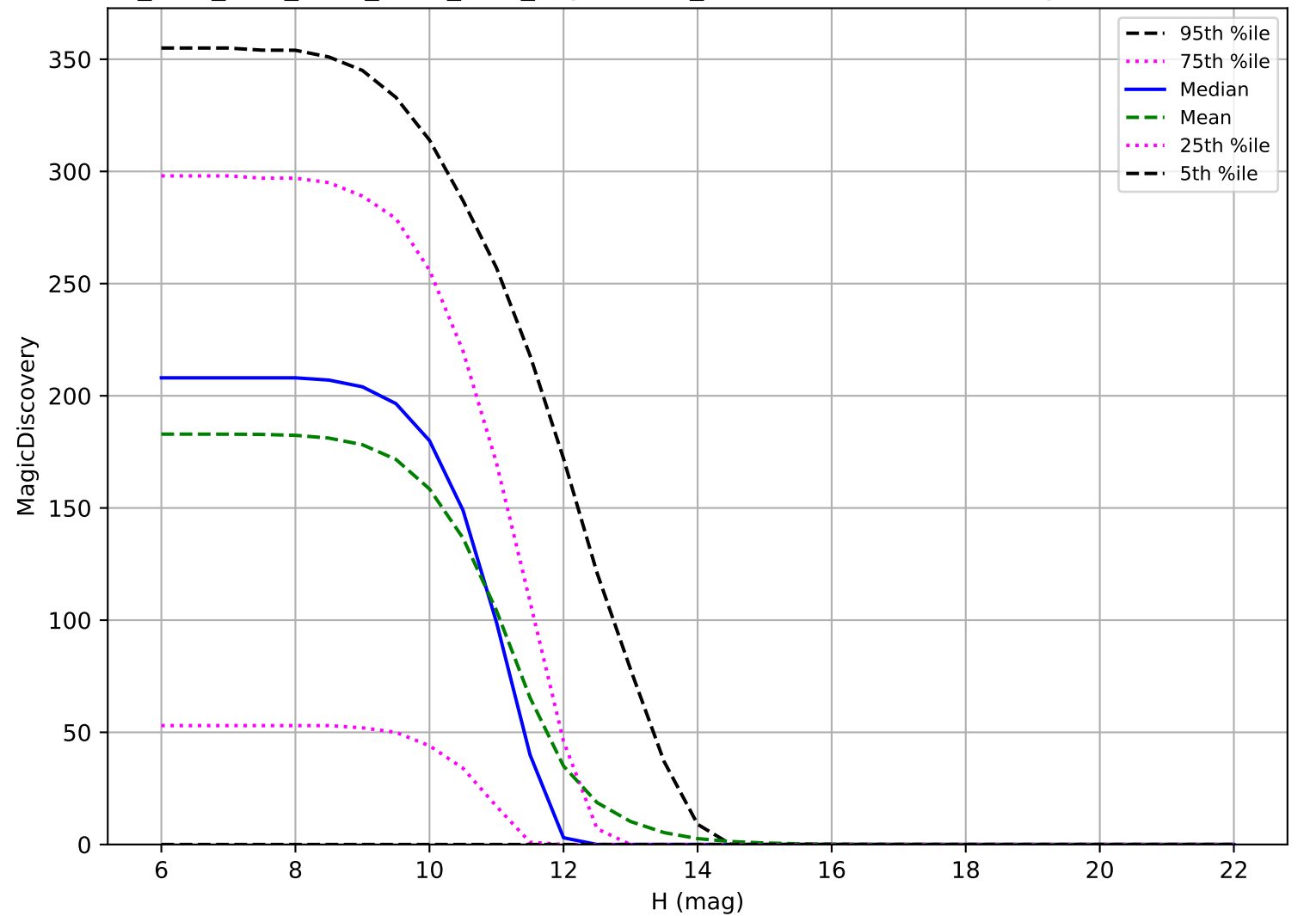
ddf_acor_sf25_lsf30_lsr10_v3.4_10yrs: OCC_r20 6 detections in 60 nights detection loss
