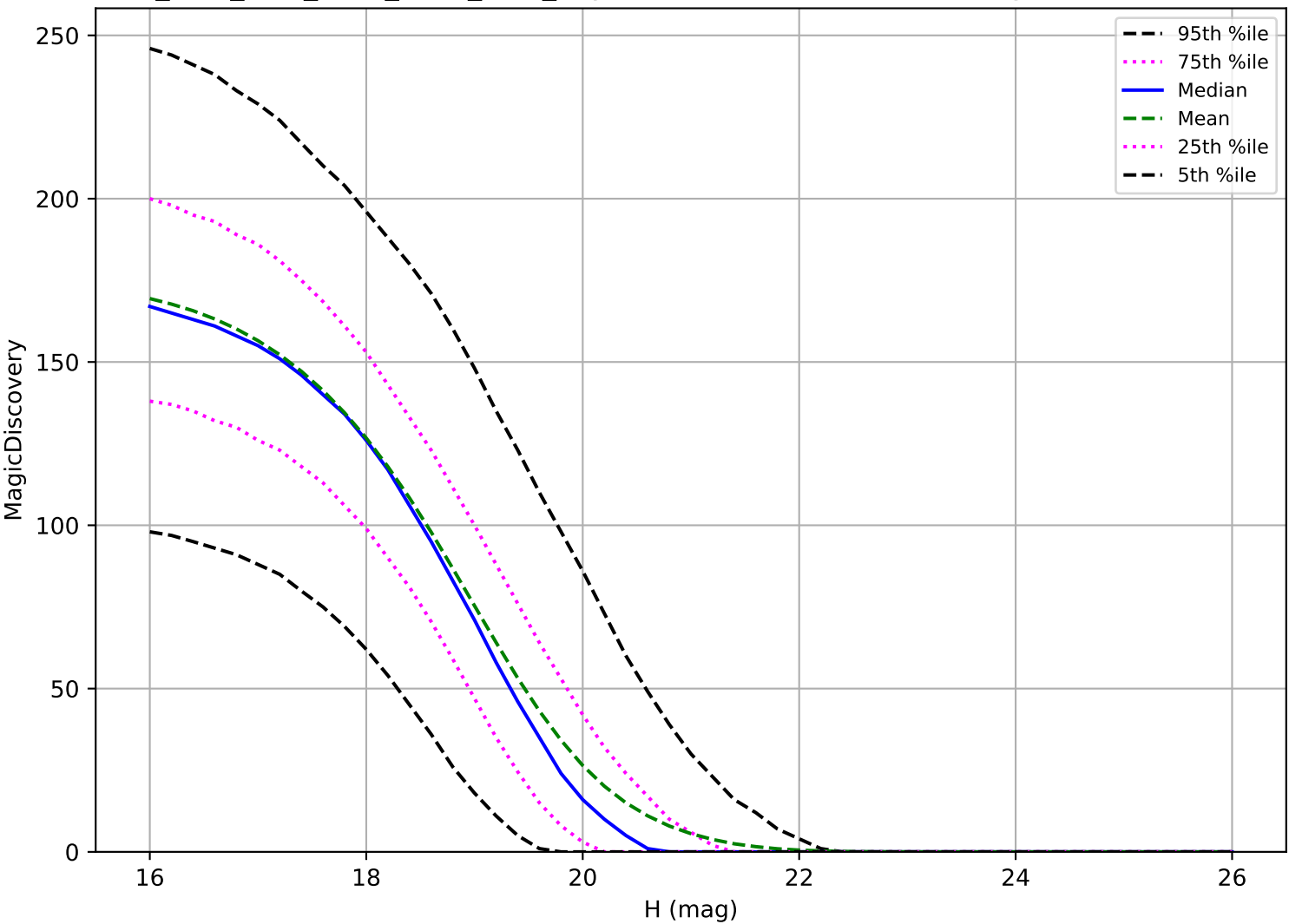
ddf_acor_sf25_lsf30_lsr10_v3.4_10yrs: MBA 6 detections in 60 nights detection loss
