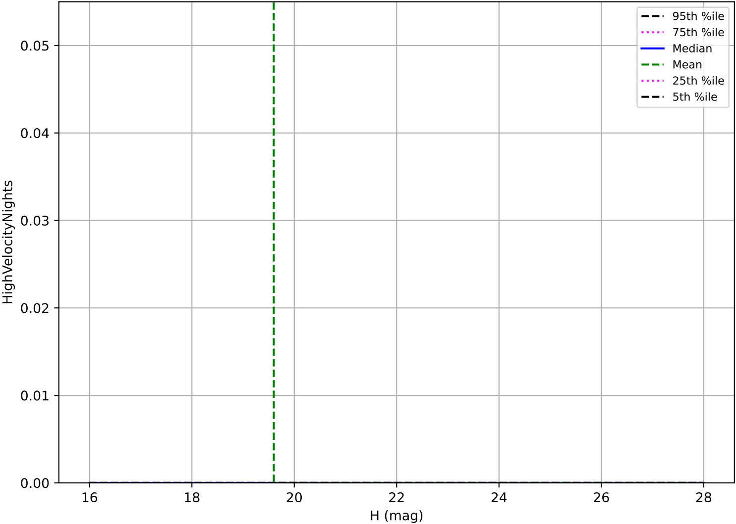
ddf_acor_sf25_lsf30_lsr10_v3.4_10yrs: Vatira High velocity pair detection loss
