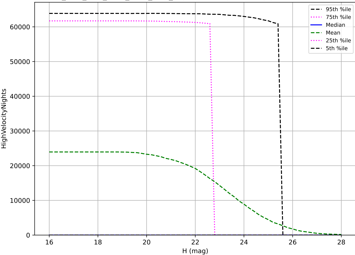
ddf_acor_sf25_lsf30_lsr10_v3.4_10yrs: PHA High velocity pair detection loss
