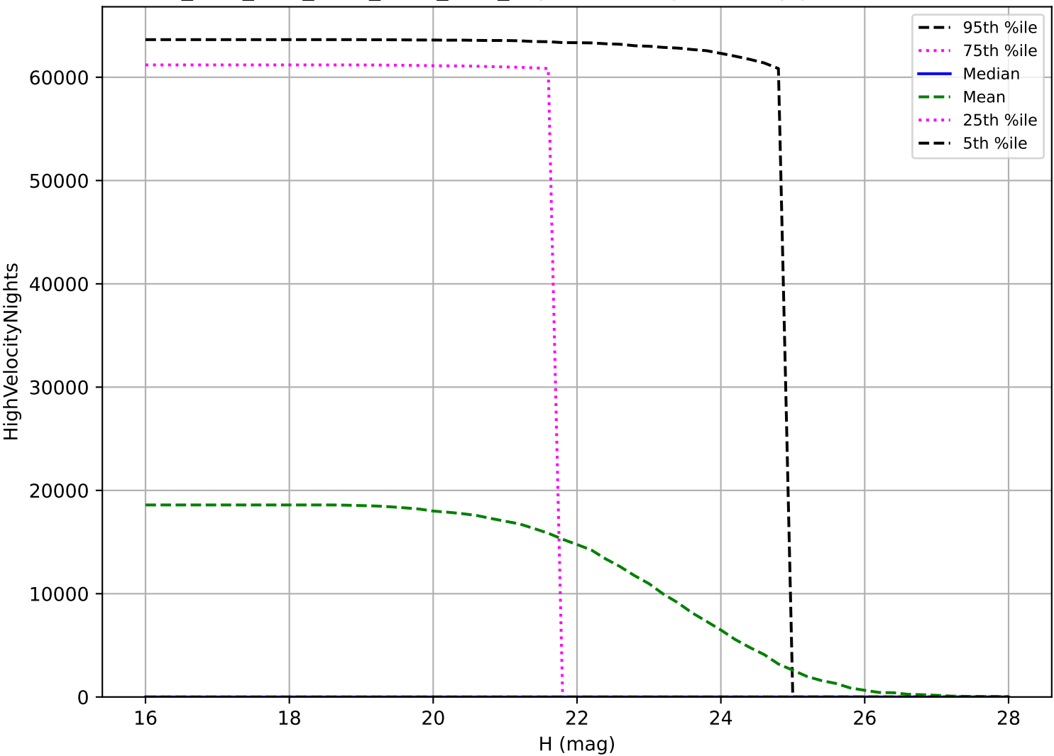
ddf_acor_sf25_lsf30_lsr10_v3.4_10yrs: NEO High velocity pair detection loss
