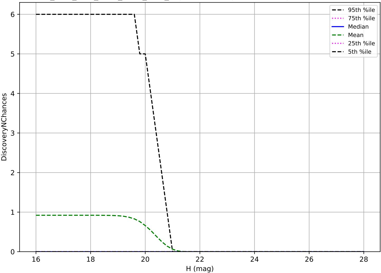
ddf_acor_sf25_lsf30_lsr10_v3.4_10yrs: Vatira 3 pairs in 15 nights detection loss
