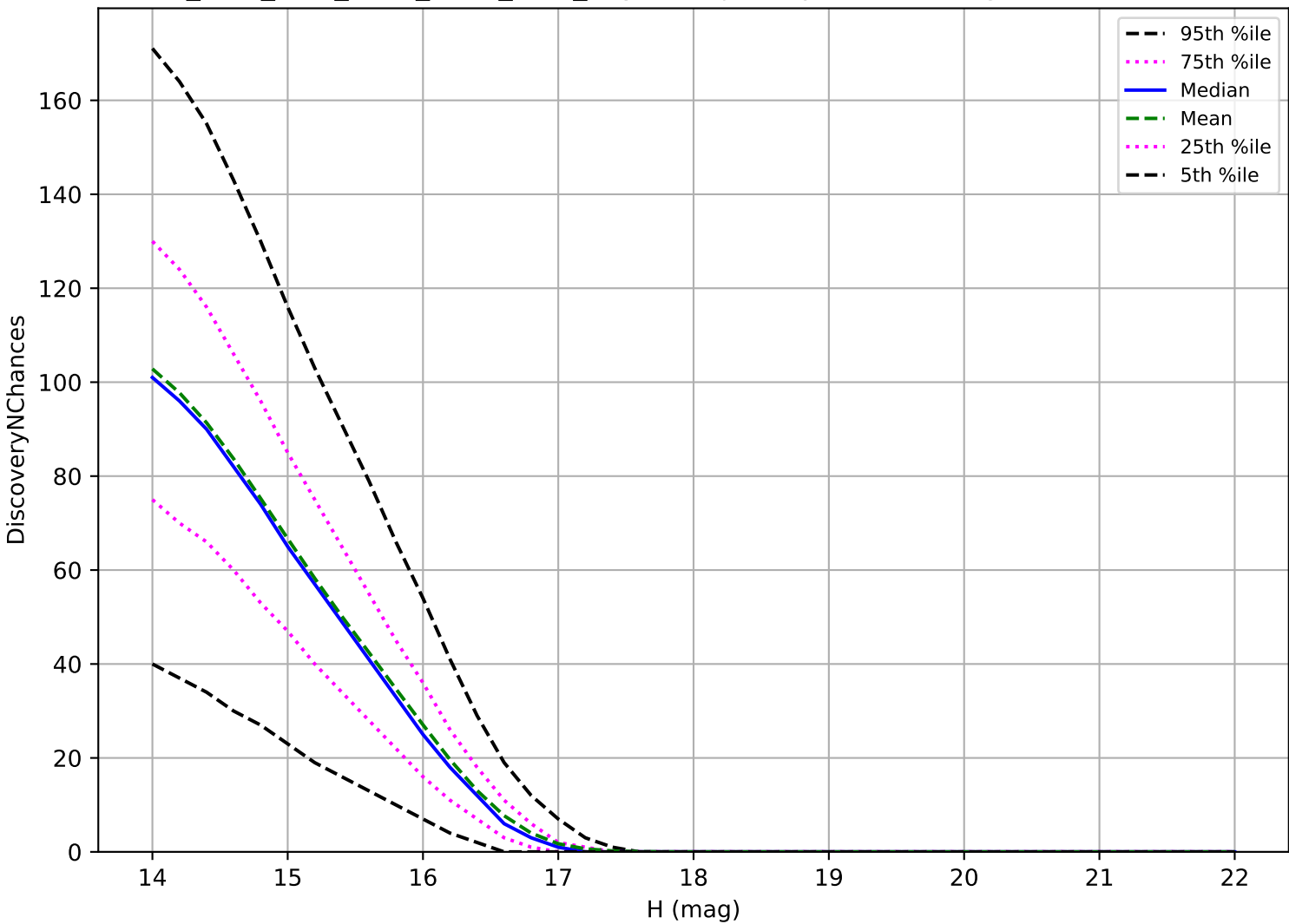
ddf_acor_sf25_lsf30_lsr10_v3.4_10yrs: Trojan 3 pairs in 15 nights detection loss
