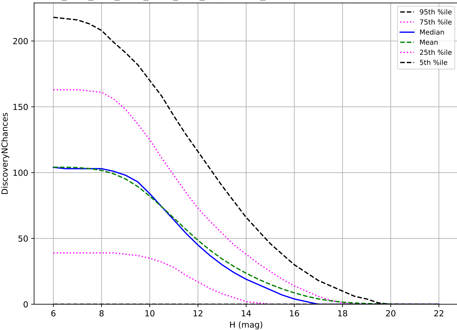
ddf_acor_sf25_lsf30_lsr10_v3.4_10yrs: OCC_r5 3 pairs in 15 nights detection loss
